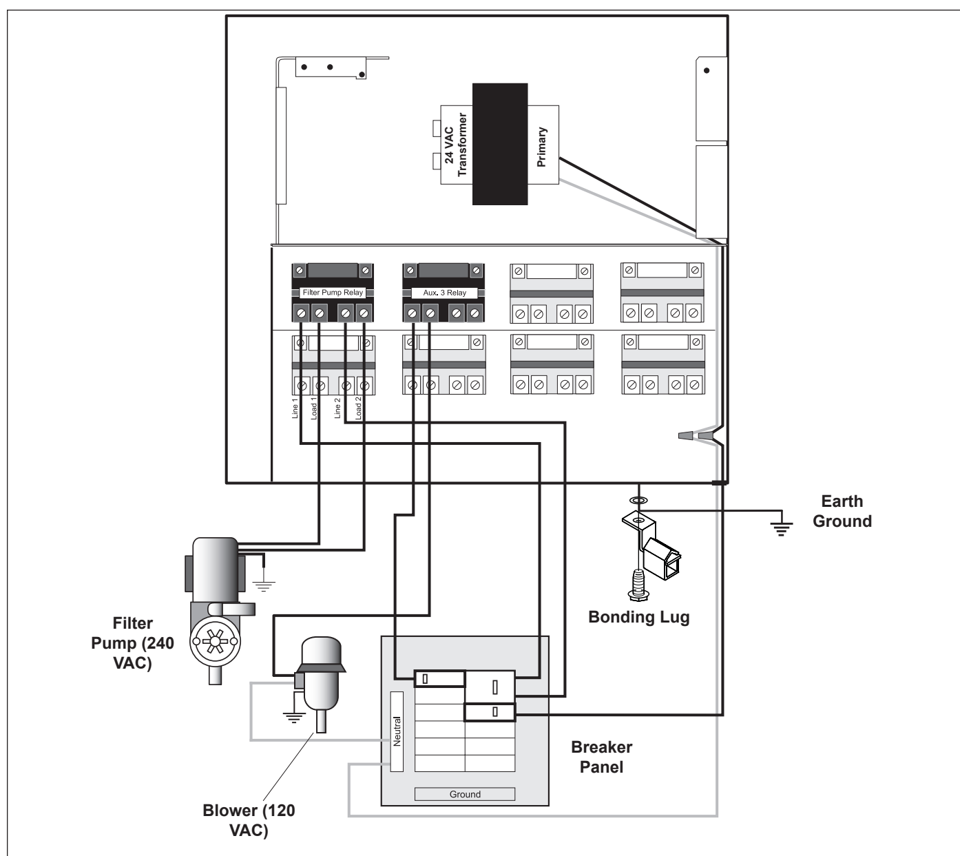
Figure 3. Standard Power Center - Bonding
