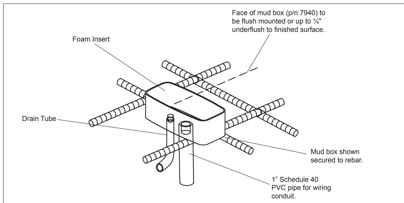
Figure 7. Horizontal Surface Rough-in Installation
