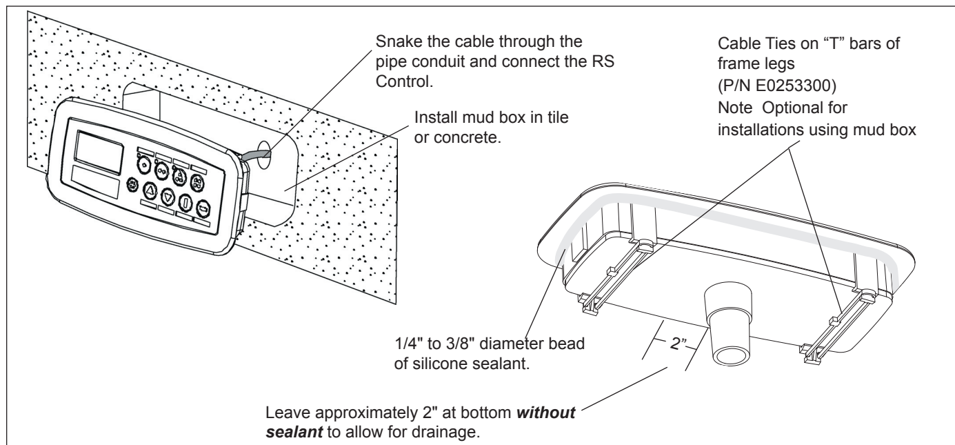
Figure 4. Vertical Installation with Optional Mud Box
