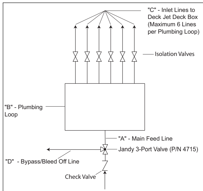
Figure 1. Multiple Jet Plumbing Diagram
