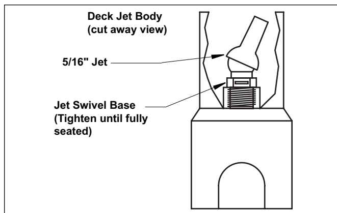
Figure 6. Snap Jet Onto Jet Swivel Base
