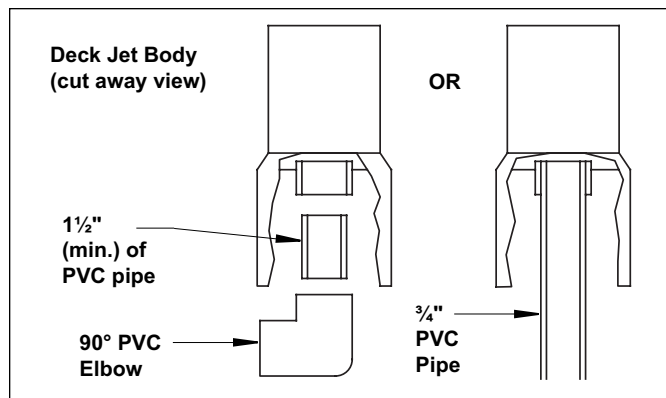
Figure 2. 90° Elbow Installation
